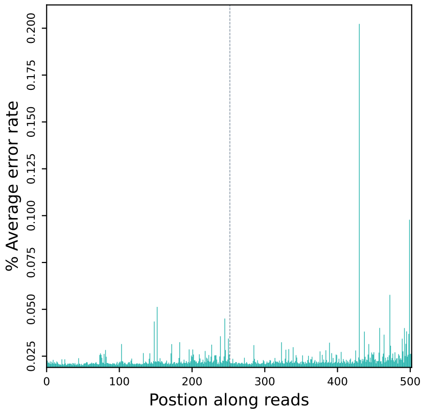
Error rate distribution along reads (R10602)
